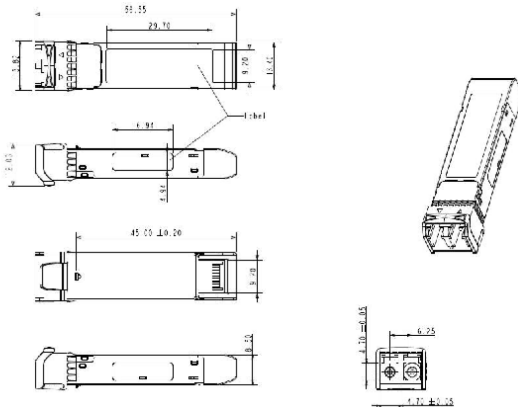
Figure 3. Mechanical Specifications
