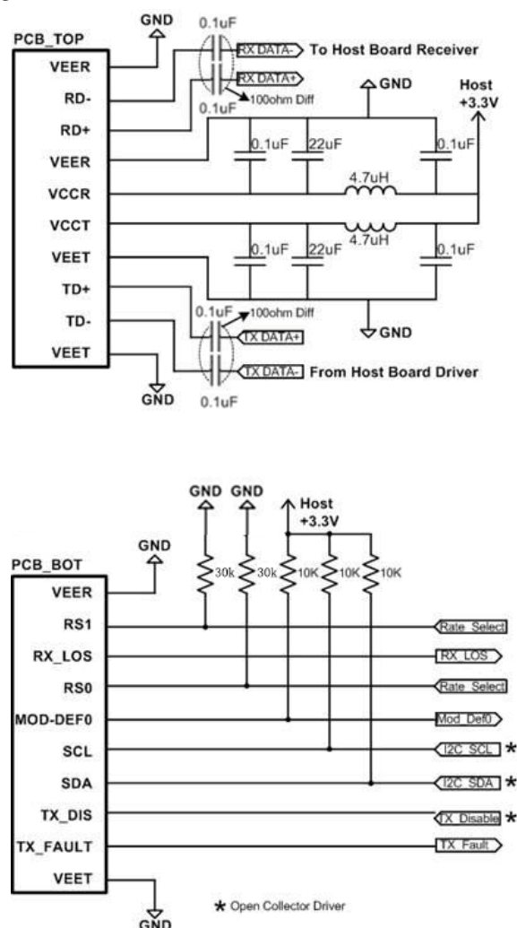
Recommended High-speed Interface Circuit
