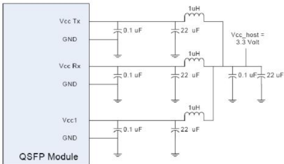
Figure 2. QSPF voltage supply and filtering scheme
