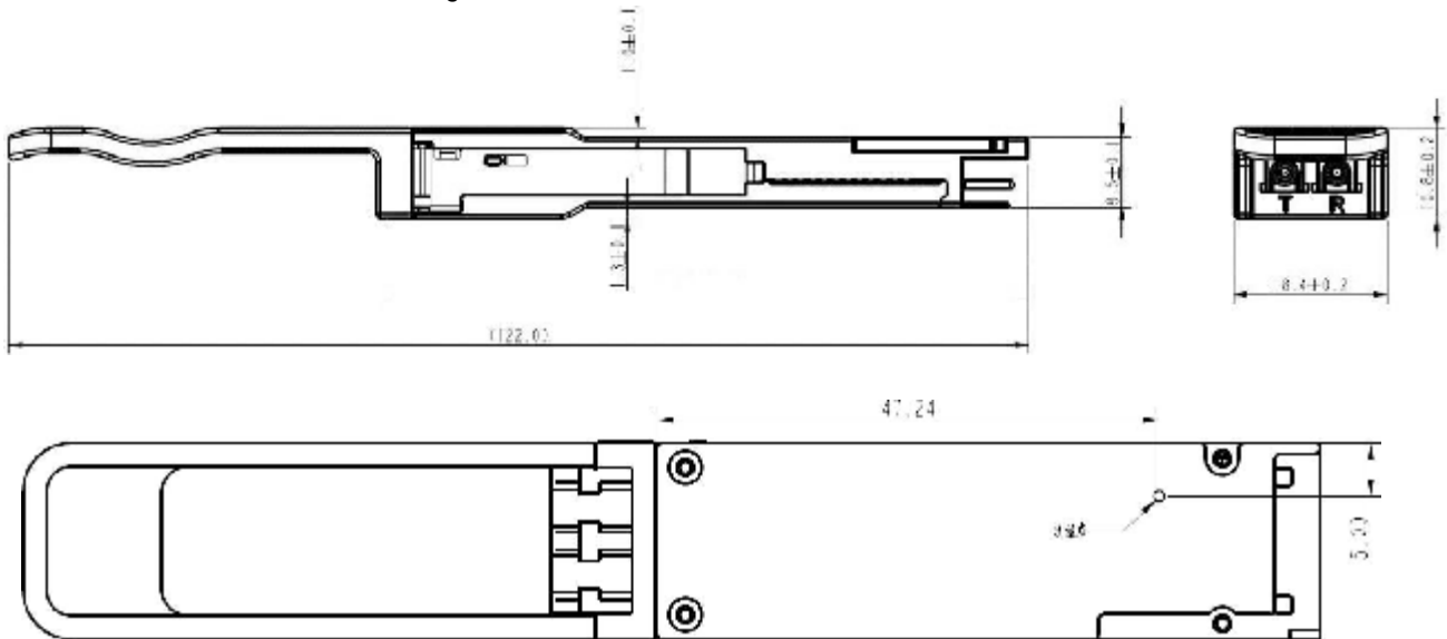
Figure 3 3C-QSFP28-FR1 Mechanical Dimensions
