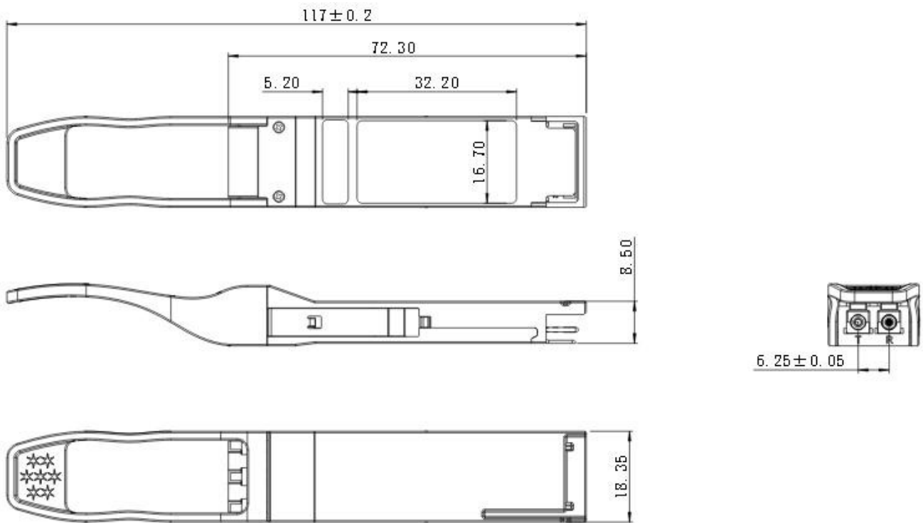
Figure 8. Mechanical Specifications
