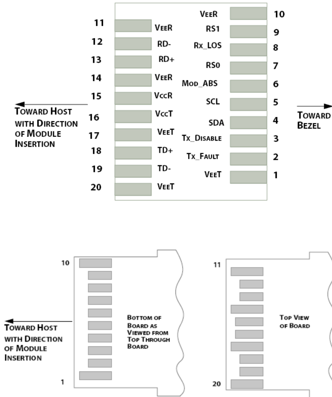
Figure2.Electrical Pin-out Details
